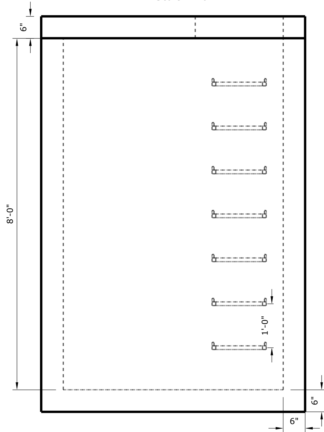
SIDE VIEW Scale 1:16
