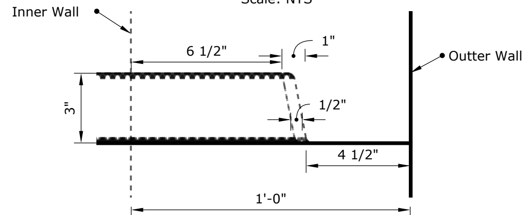
1' Pallet and Header Joint Detail
